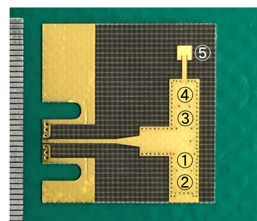
Substrate with \epsilon_r=2.2 and thickness t=0.127 mm
