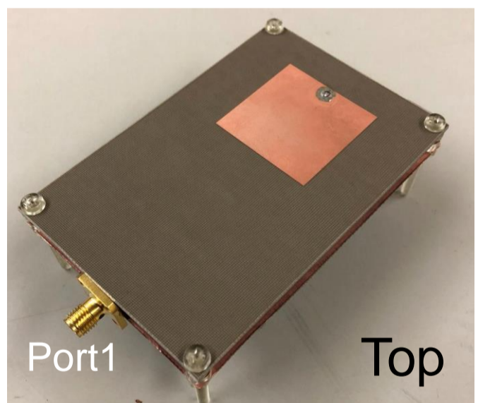
Substrate with \epsilon_r=2.6 and thickness t=1.0 mm
