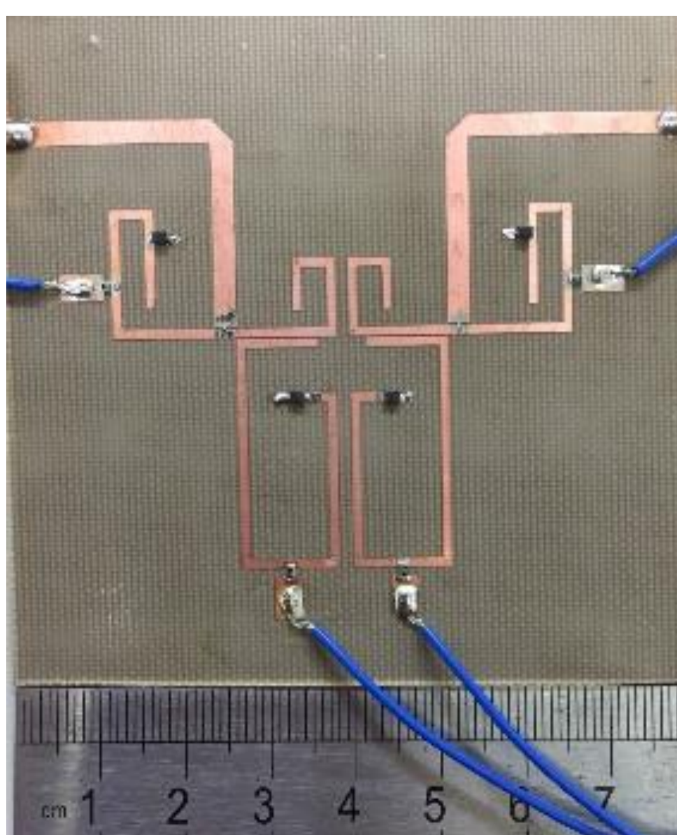
Substrate with \epsilon_r=2.81 , thickness t=1.0\text{mm}
