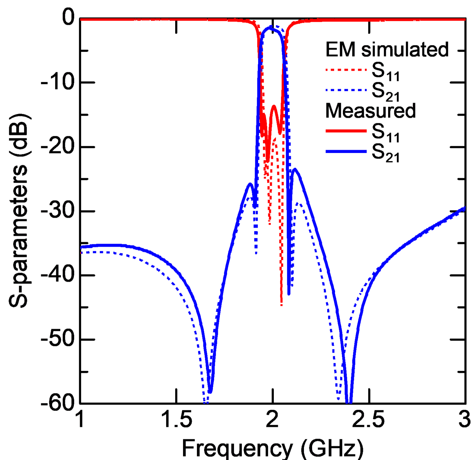
4段Cul-de-Sac結合BPF ( f_0=2\text{ GHz} , \Delta f=100\text{ MHz} )
