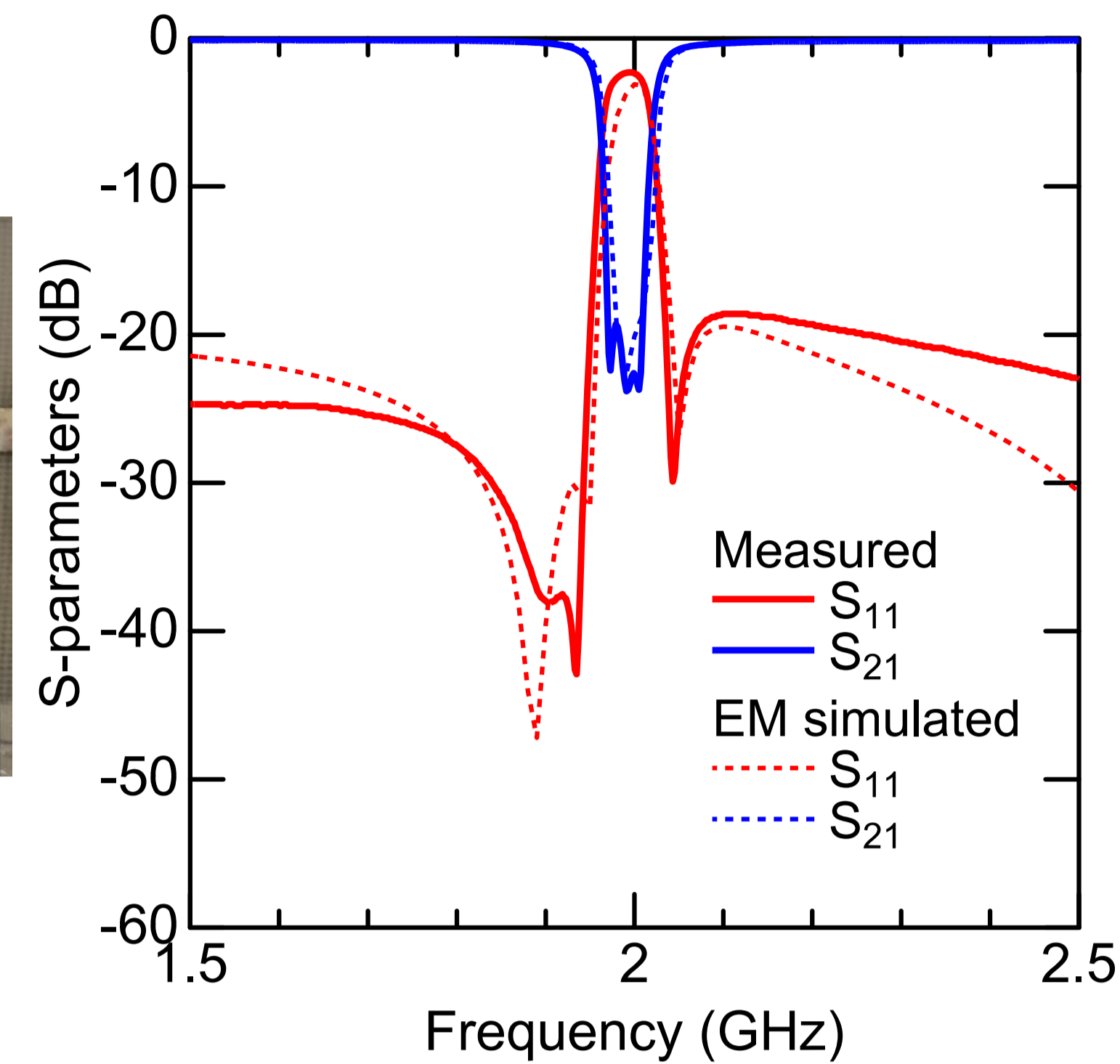
3段Cul-de-Sac結合BSF ( f_0=2\text{ GHz} , \Delta f=40\text{ MHz} )
