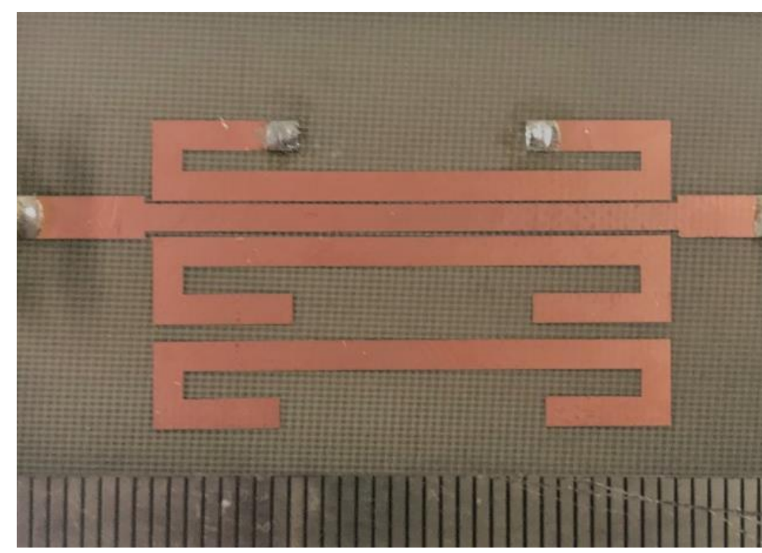
Substrate with \epsilon_r=2.6 and thickness t=1.0\text{mm}
