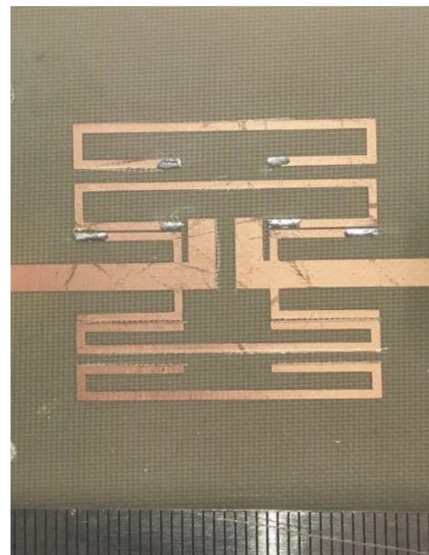
Substrate with \epsilon_r=2.6 and thickness t=1.0\text{mm}
